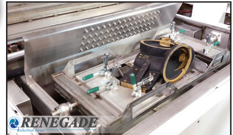
Rotary Fixture Assembly with Spray Manifold
