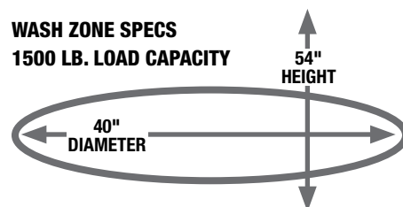
Heavy Duty Gear-Driven Turntable Assembly
